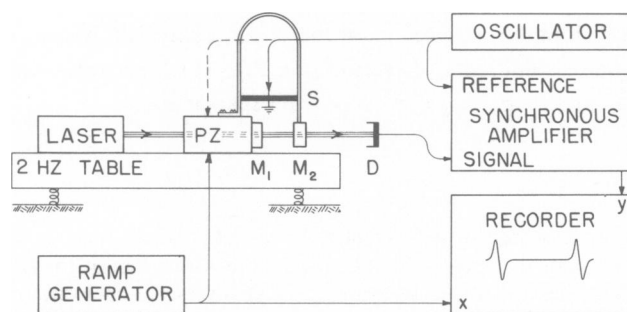
FIGURE 2 Differential Perot-Fabry interferometer M_1M_2 for measuring small piezoelectrically induced deformations in sample S . The synchronous amplifier rectifies the signal from the photodetector D in synchronism with the sinusoidal voltage from the oscillator. The piezoelectric translator PZ slowly moves mirror M_1 through conditions for interference (two such conditions shown on the recorder). The translator is also used to calibrate the sensitivity of the system (substitutional connection shown by dashed line).
