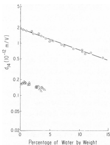
FIGURE 3 The piezoelectric constant of bovine tendon (upper points) and bone (lower points). The perfect exponential decrease signifies a random transitory cancellation of electric dipoles by water molecules. The slope of the upper line may place limits on the average molecular weight of the amino acid residual responsible for piezoelectricity in collagen.
